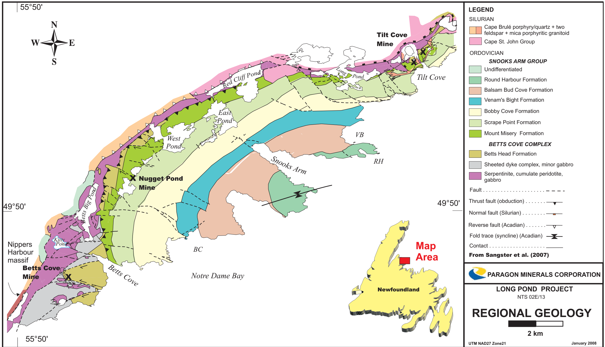
Figure 3. Geology of the Bett's Cove Area, Baie Verte Peninsula.
