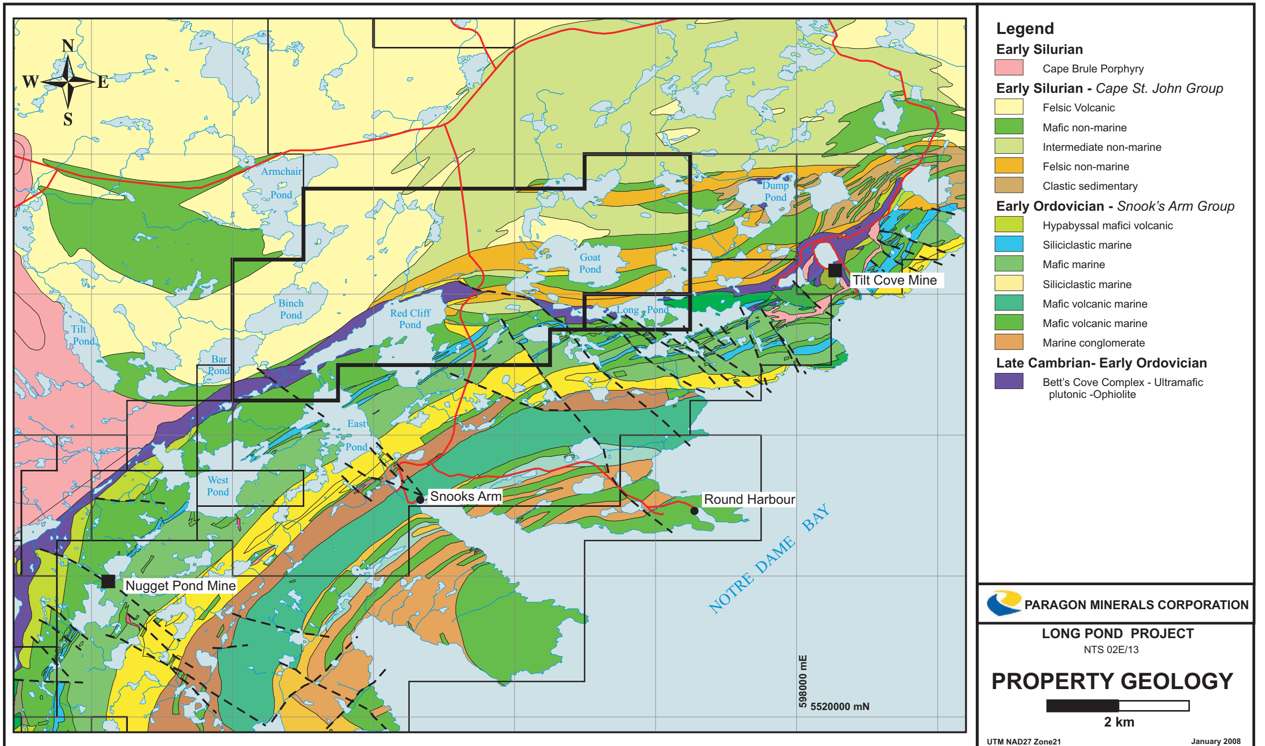
Figure 4. Property Geology, Long Pond area, Baie Verte Peninsula.
